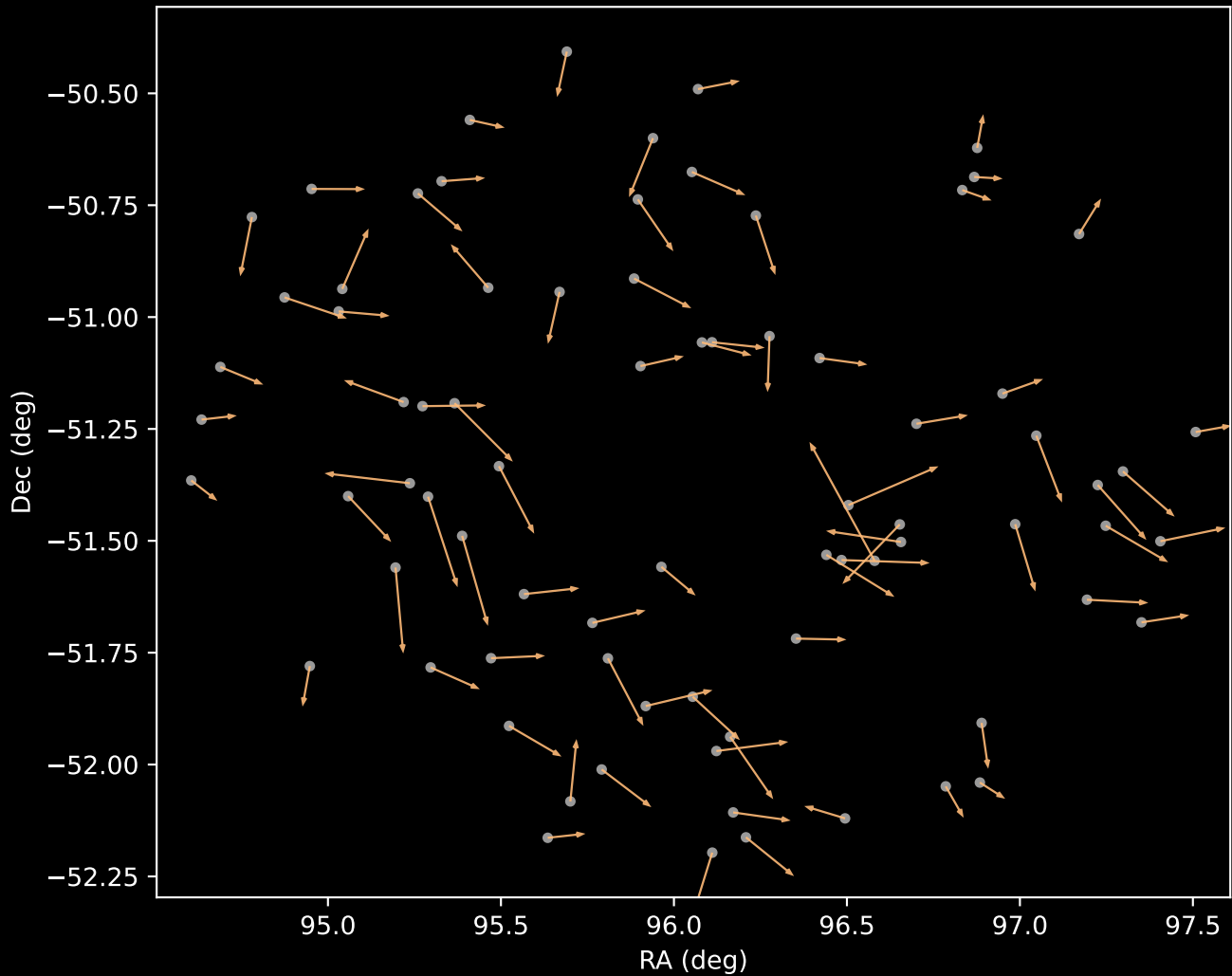
APOGEE DR17 Cluster 3 Proper Motion Vectors (n=78)
