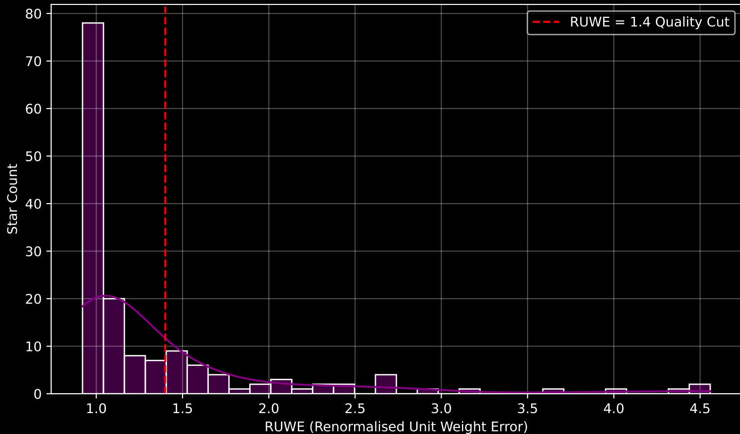
GAPOGEE DR17 Field [JHelium5] RUWE Distribution (n= 154)
