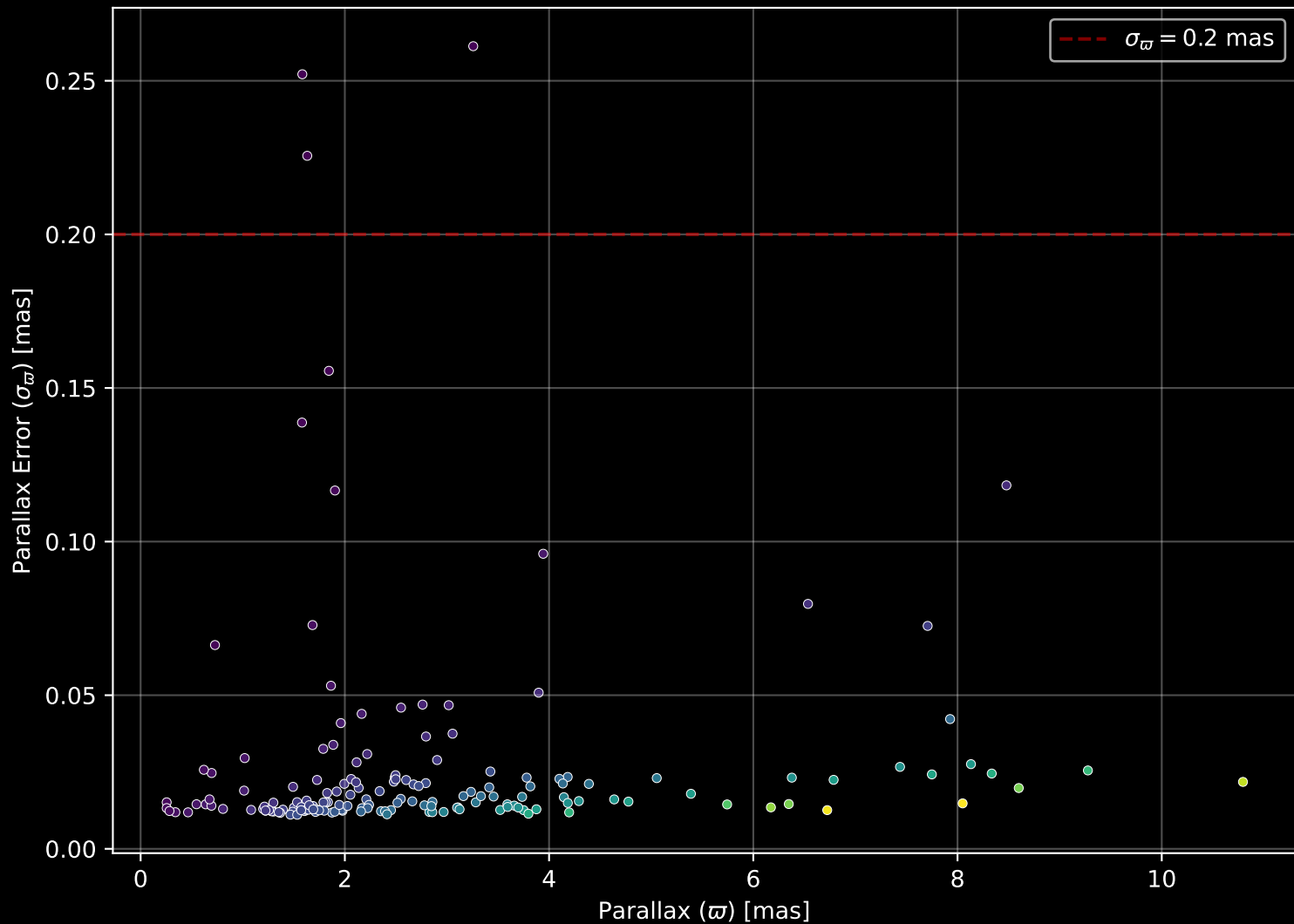
APOGEE DR17 Field: [JHelum5] Parallax Quality (n= 165)
