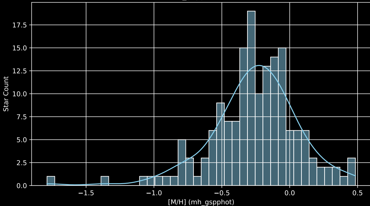
APOGEE DR17 Field: [JHelum5 [M/H] (mh_gspphot) (n= 165)
