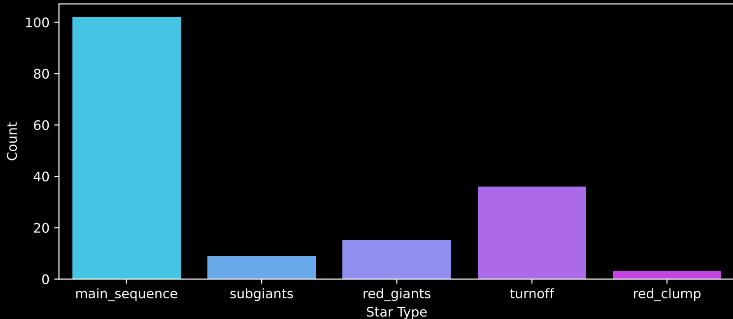
APOGEE DR17 Field: [JHelum5] Count plot of Star Type
