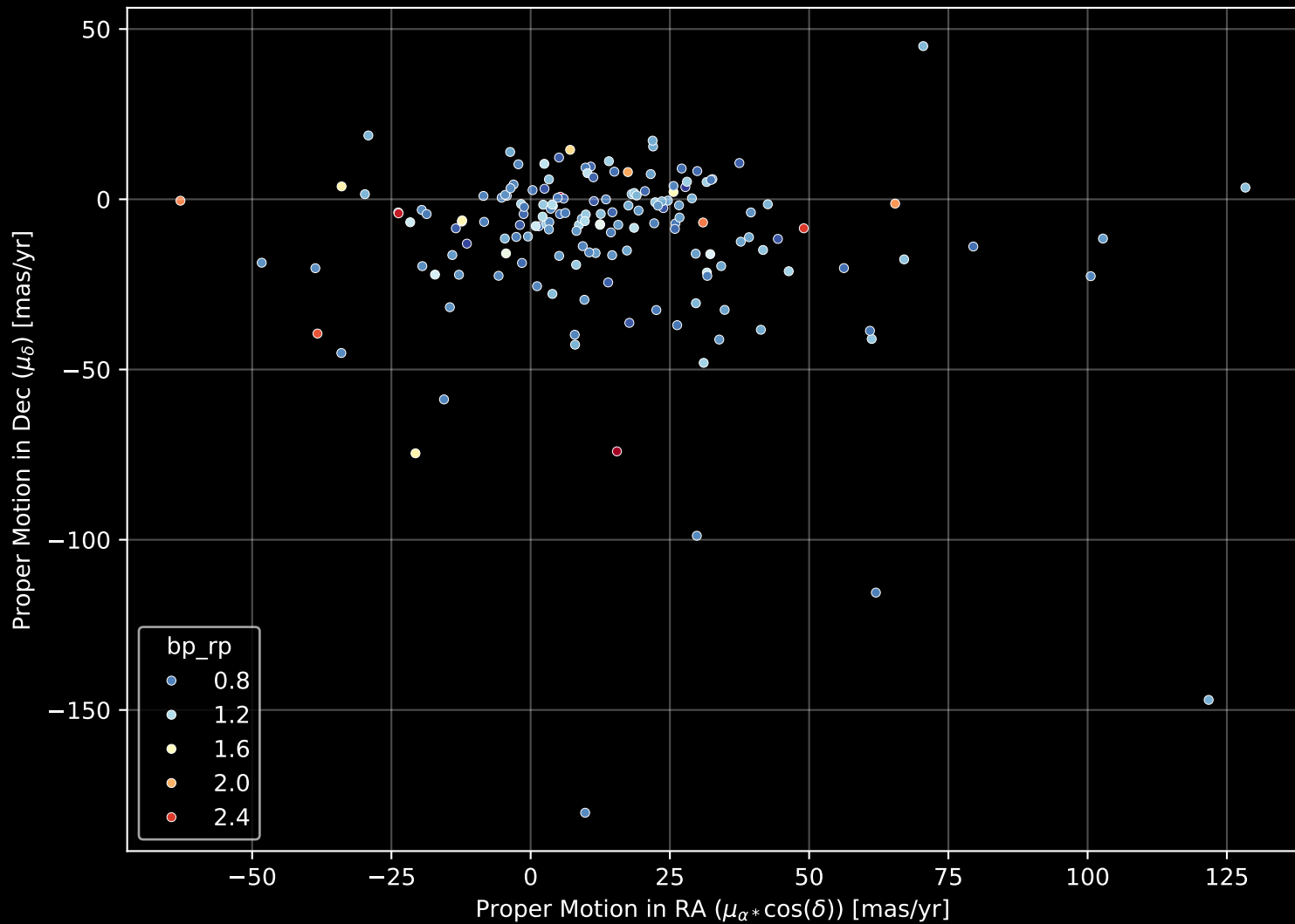
APOGEE DR17 Field: [JHelium5] Proper Motion Diagram (n= 165)
