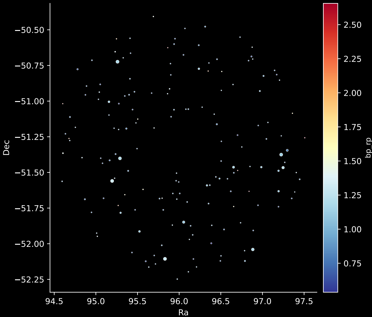
APOGEE DR17 Field: [JHelum5] Stars: 165
